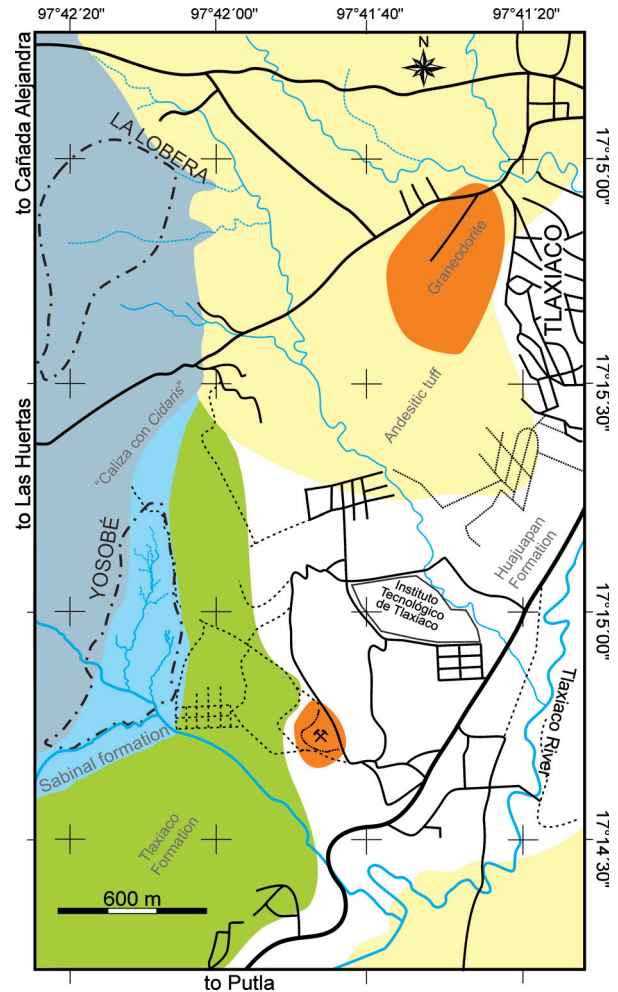
FIGURE 3. Geologic map of Tlaxiaco showing the position and shape of Yosobé and La Lobera localities (modified from SGM 2000a, 2000b, 2009).
