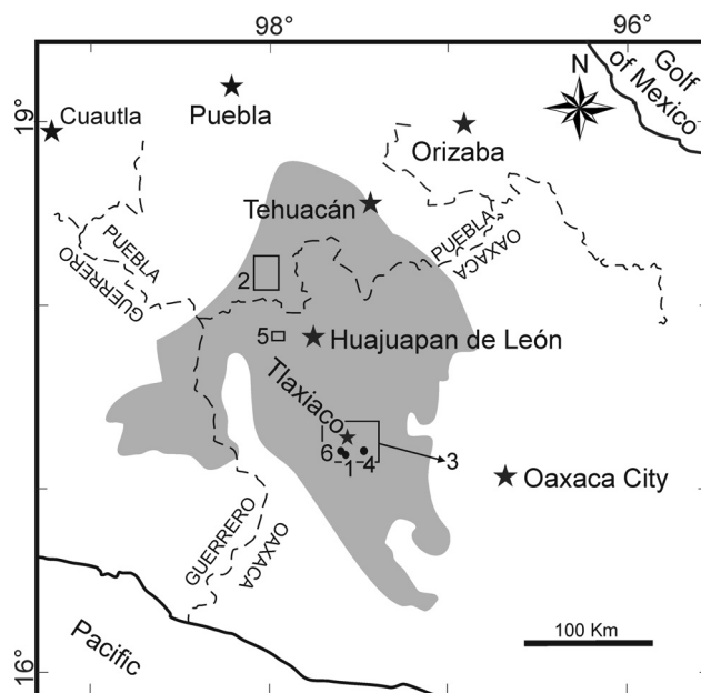
FIGURE 2. Map of the Tlaxiaco Basin and distribution of the vertebrate fossil localities and areas reported before the present manuscript. 1, Cerro de la Virgen; 2, Petalcingo area; 3, Wieland's area; 4, Amoltepec area; 5, Papalutla; 6, La Lobera; 7, Yosobé (6 and 7 are new localities reported in the present paper).
