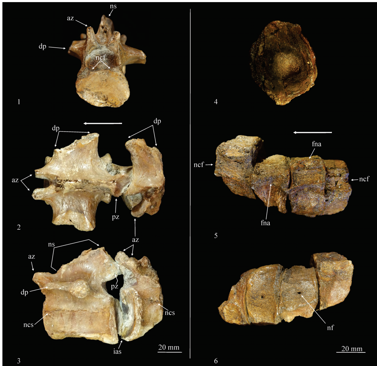
FIGURE 10. Vertebrae of marine reptiles from Yosobé. 1-3, Specimen IGM 9324, undetermined thalattosuchian crocodyliform in anterior (1), dorsal (2), and lateral (3) views. 4-6, Specimen IGM 9325, undetermined optalmosaurid ichthyosaur in anterior (4), dorsal (5), and ventral (6) views. In both specimens the arrows show the anterior direction. Abbreviations: dp, diapophyseal process; fna, facet for the neural arch; ias, intervertebral articular surfaces; ncf, neural canal floor; ncs, neurocentral suture; nf, nutritive foramen; ns, neural spine; pz, posterior zygapophysis.
